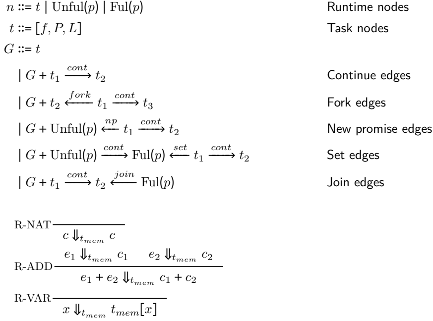
■ Figure 3 Computation graph and reduction rule
