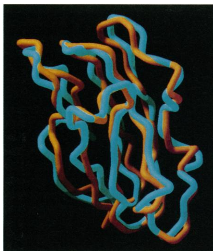
Fig. 1. The NMR solution structure of french bean plastocyanin in red and the corresponding superimposed lattice fit of apoplastocyanin in blue.
