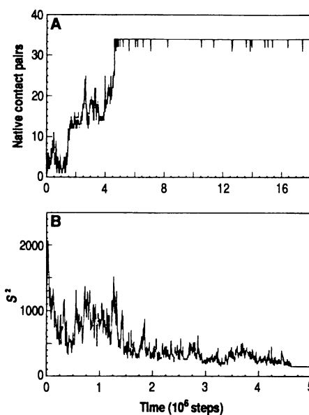
Fig. 3. For a representative folding trajectory, (A) a plot of the number of contacts between pairs of side chains versus time and (B) the instantaneous value of the square of the radius of gyration S^2 versus time.
