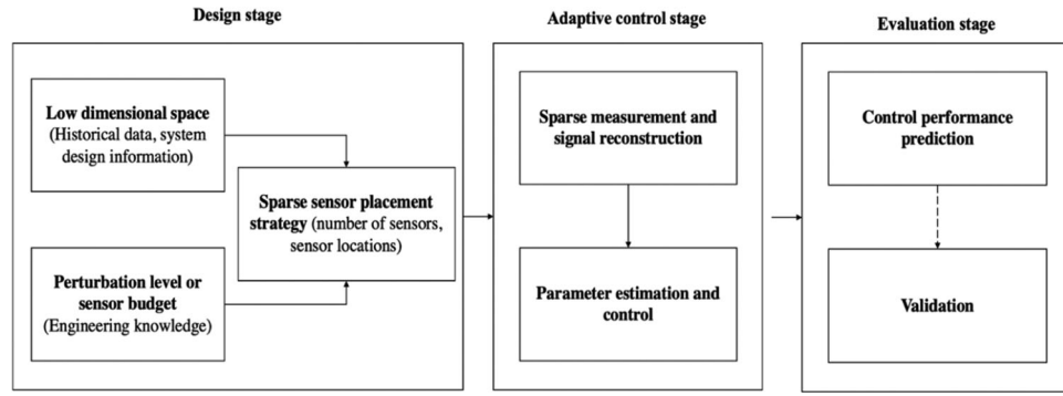
Figure 2. An overview of the proposed SPAC method.
