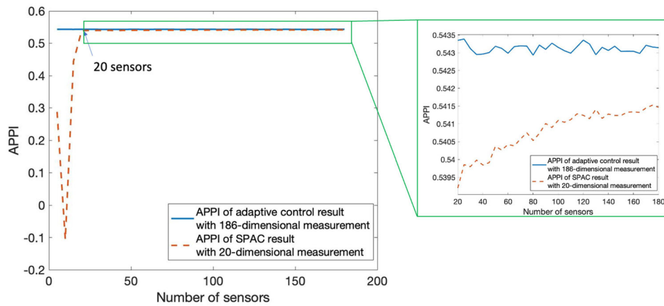
Figure 8. Sensitivity analysis of the SPAC method by varying the number of sensors.
