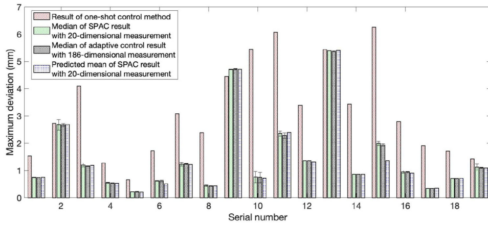
Figure 7. Comparison among the one-shot control, the adaptive control with 186-dimensional measurement, and the SPAC with 20-dimensional measurement.
